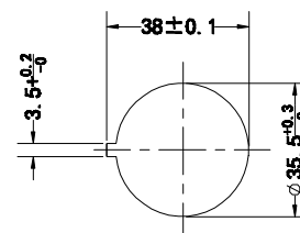
Mounting hole dimensions
