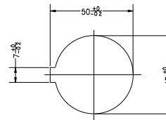
Mounting hole dimensions
