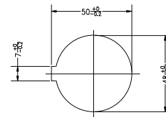
Mounting hole dimensions
